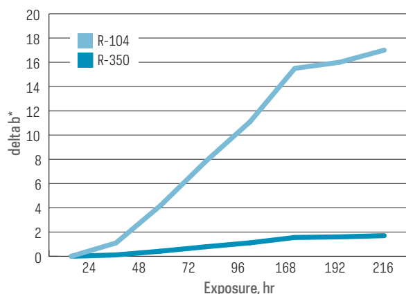
Figure 3. Polyethylene Discoloration
